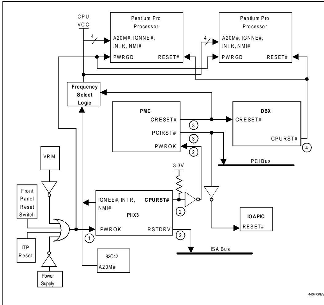
Figure 13. Reset Structure for 440FX PCiset with PIIX3
